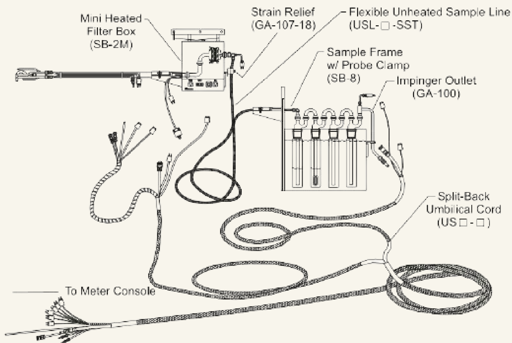
Schematic of Method 5 Flexible Sampling Train
